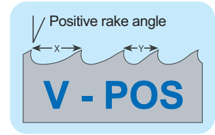
Variable tooth with positive hook angle
