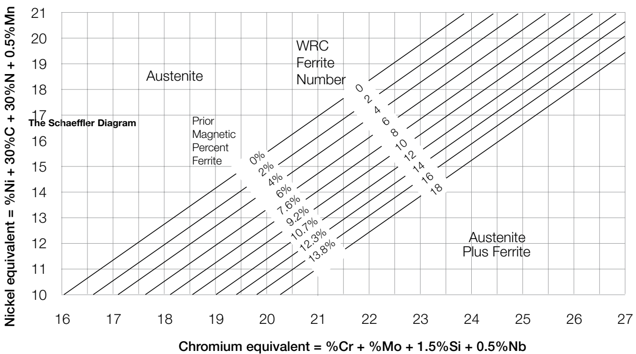
The DeLong Diagram
