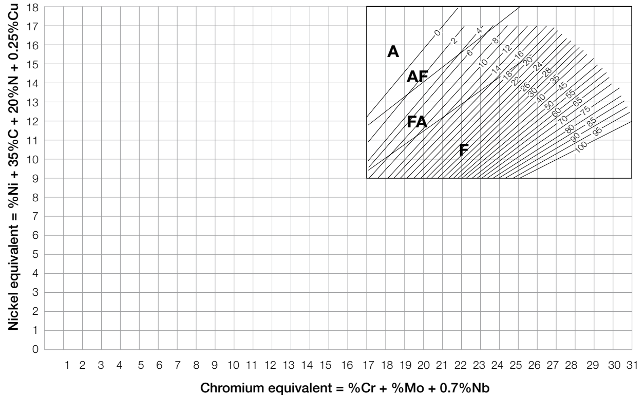
the WRC-1992 diagram (see Figures Z and W)
