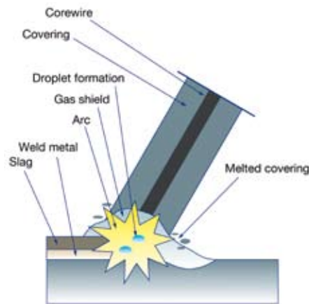
Principle of manual metal arc welding.
