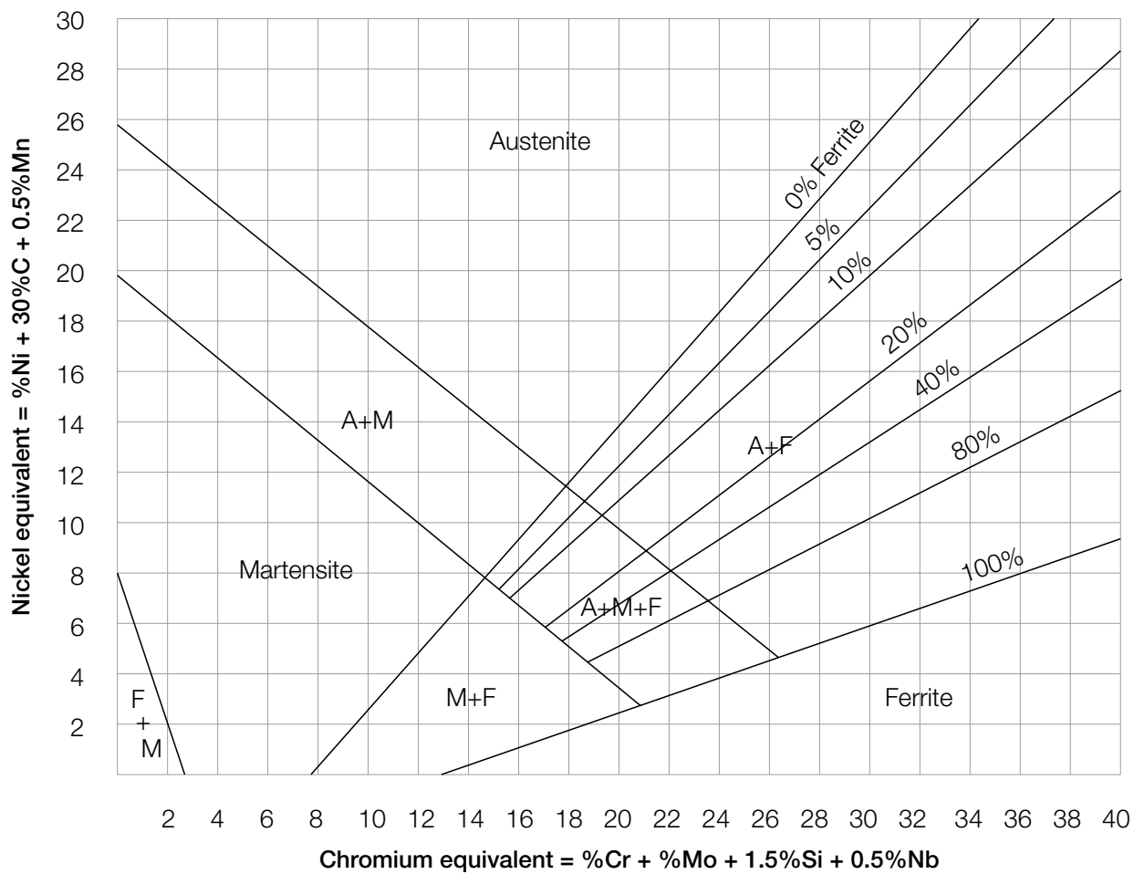
The Schaeffler Diagram
